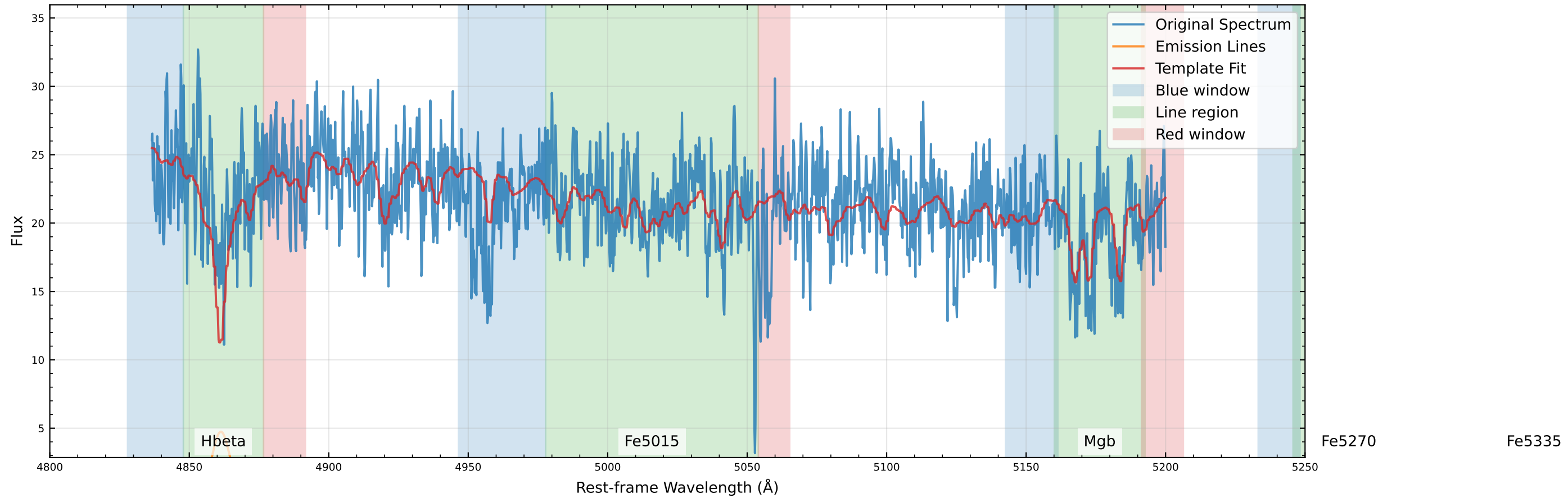
Original Data Comparison ( v_{\text{star}}=7.8 km/s, v_{\text{gas}}=-45.6 km/s)
