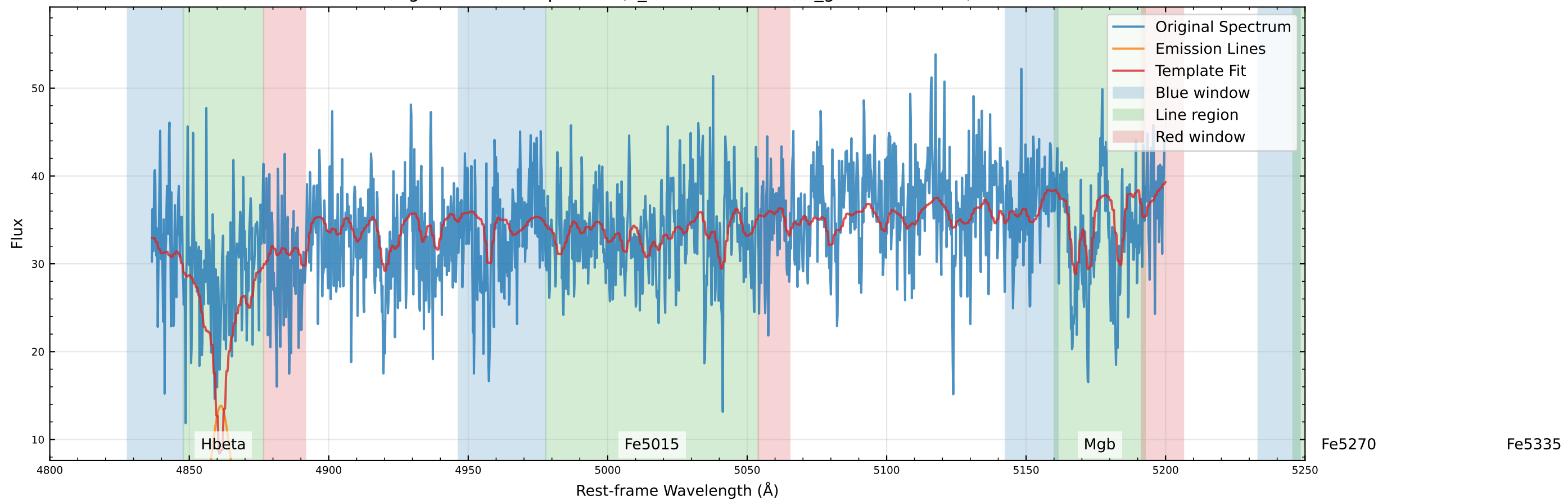
Original Data Comparison ( v_{\text{star}}=-38.7 km/s, v_{\text{gas}}=-60.9 km/s)
