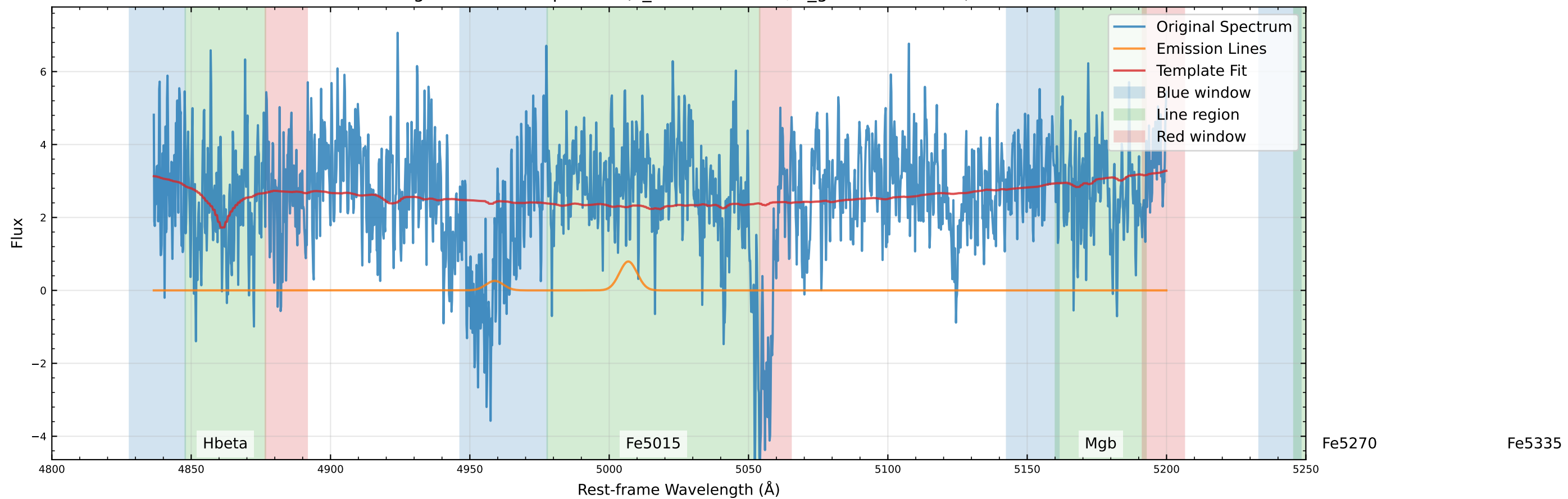
Original Data Comparison (v_star=-2.5 km/s, v_gas=291.3 km/s)
