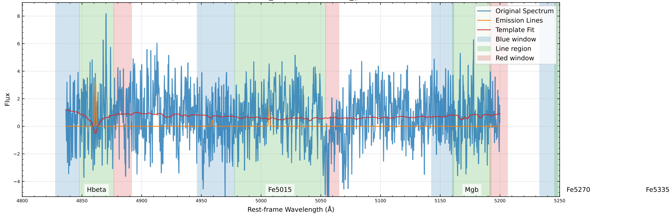
Original Data Comparison (v_star=-214.2 km/s, v_gas=-278.3 km/s)
