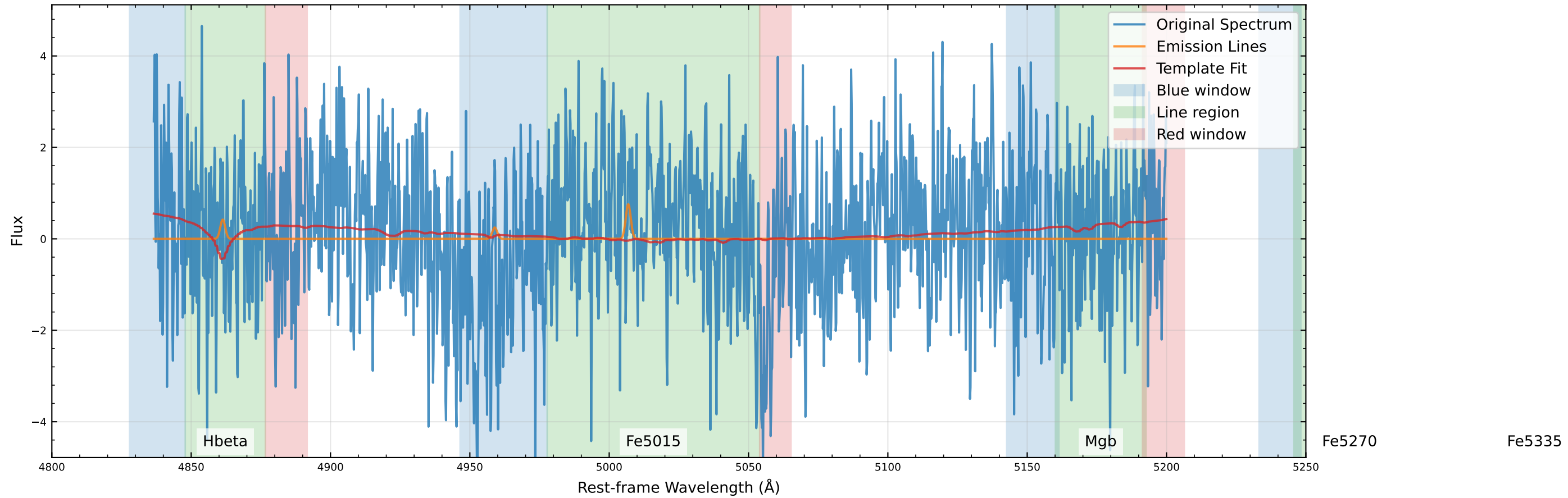
Original Data Comparison (v_star=-98.4 km/s, v_gas=-91.0 km/s)
