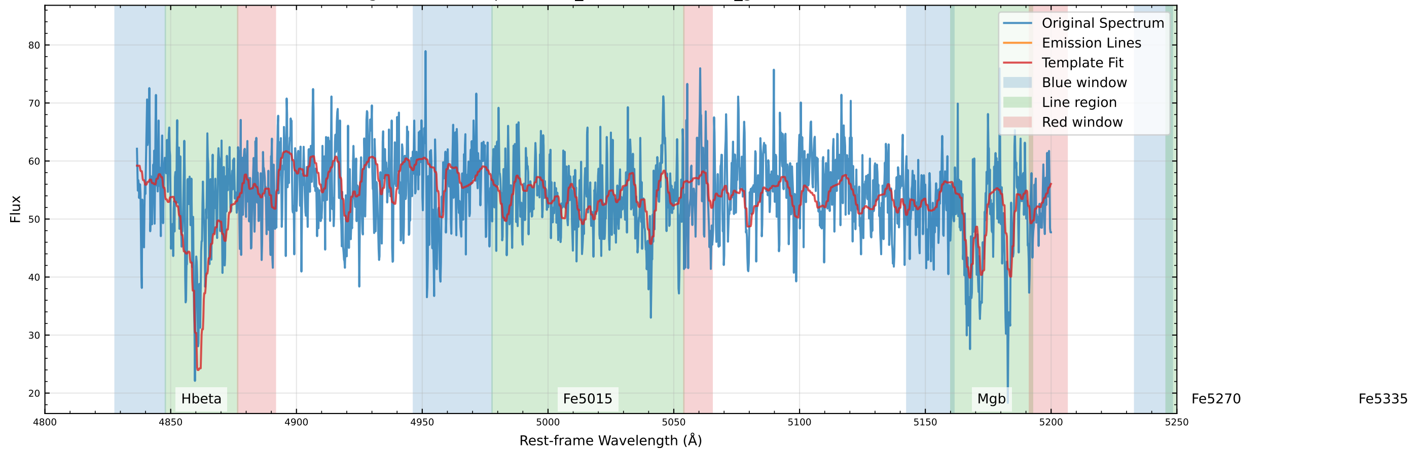
Original Data Comparison (v_star=-39.3 km/s, v_gas=-16.7 km/s)
