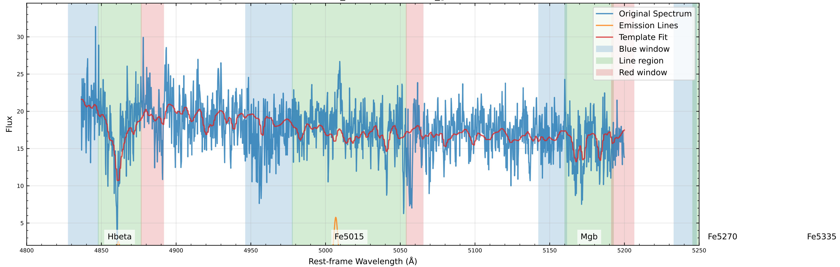
Original Data Comparison (v_star=-55.1 km/s, v_gas=144.0 km/s)
