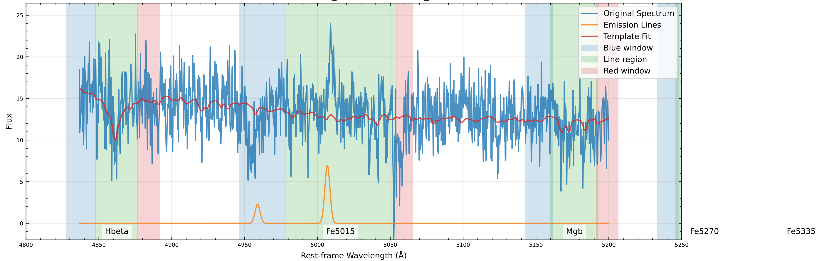
Original Data Comparison (v_star=-37.1 km/s, v_gas=166.4 km/s)
