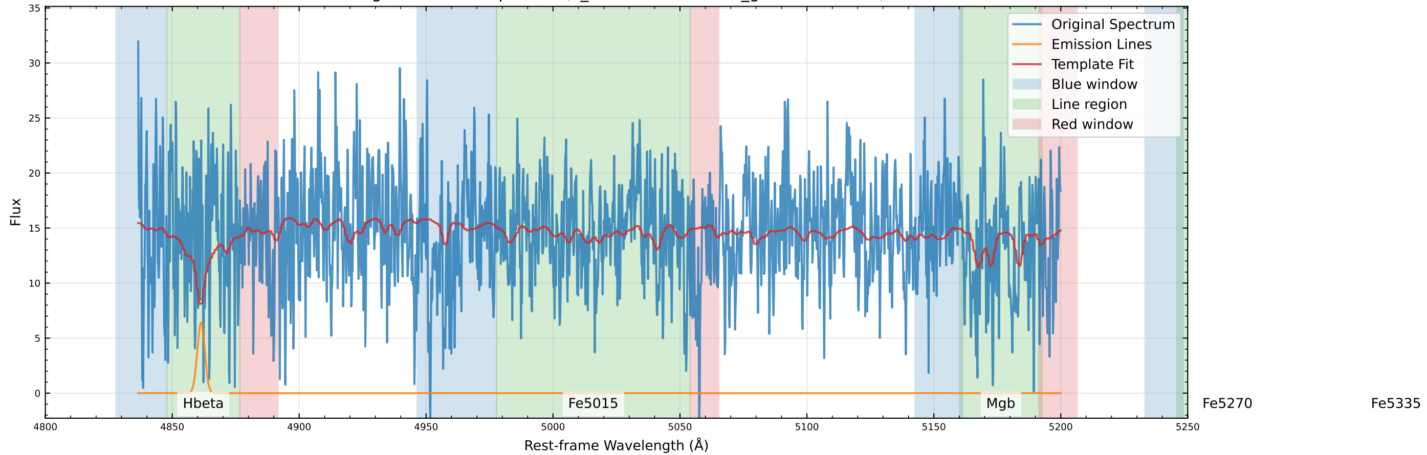
Original Data Comparison (v_star=-49.9 km/s, v_gas=-75.4 km/s)
