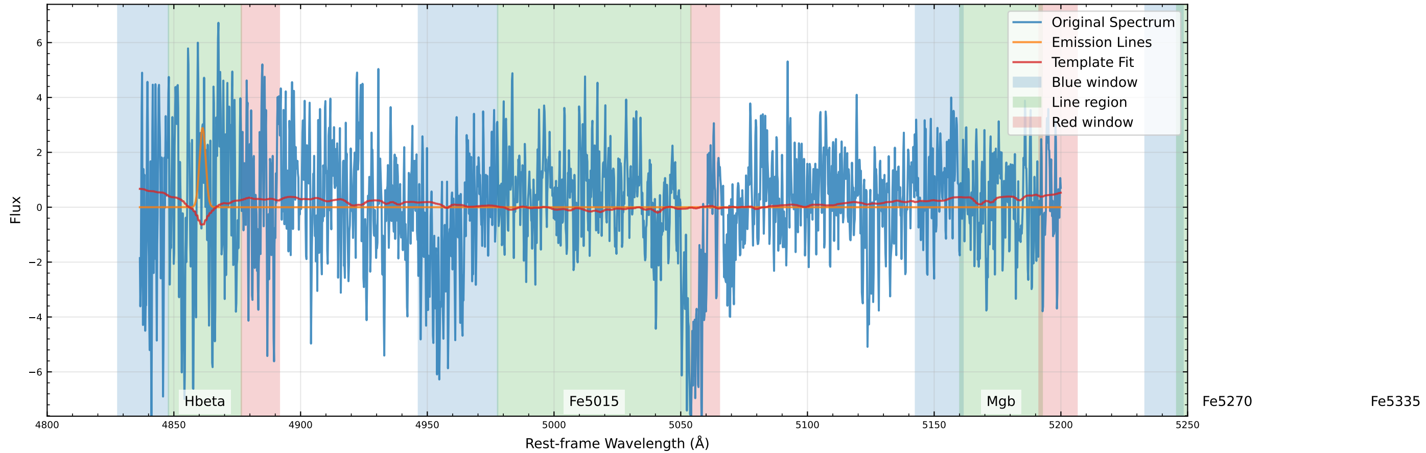
Original Data Comparison (v_star=-43.1 km/s, v_gas=-36.0 km/s)
