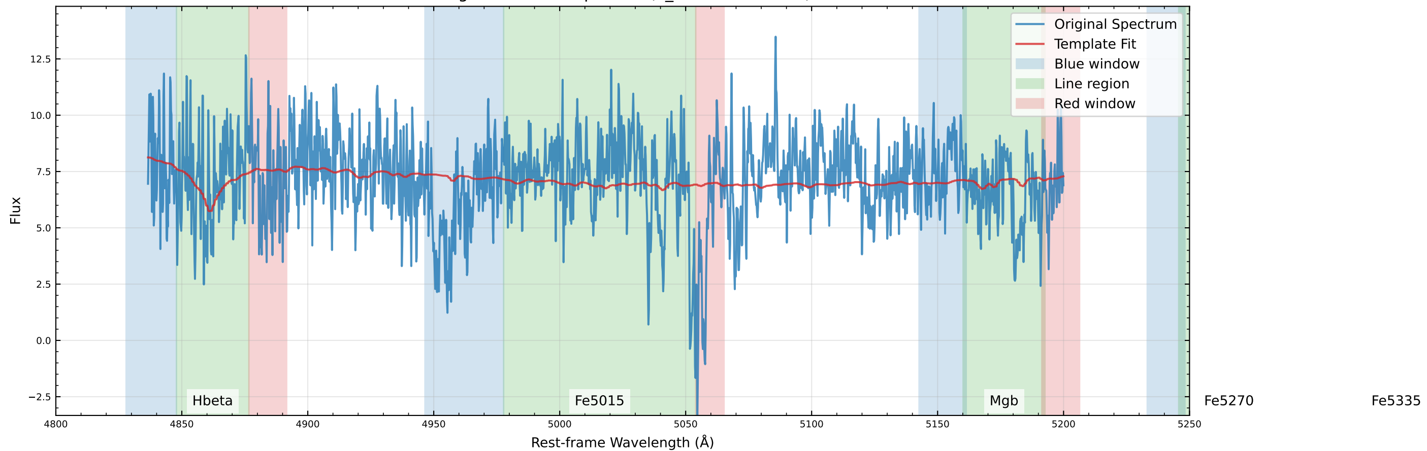
Original Data Comparison (v_star=-69.4 km/s)
