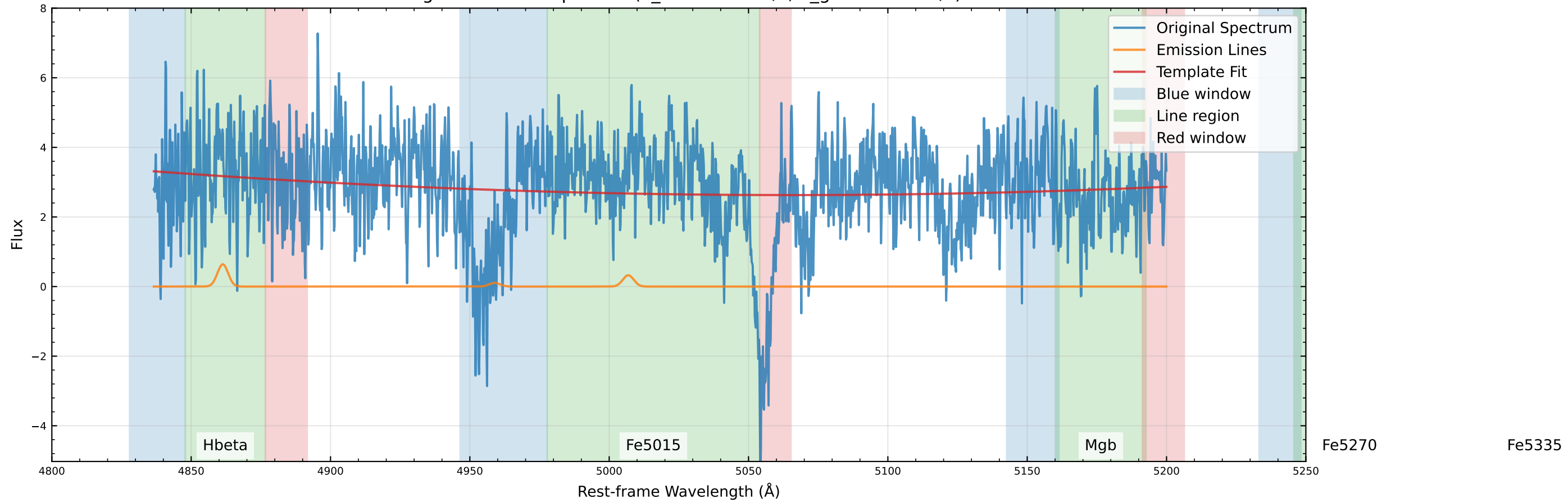
Original Data Comparison (v_star=3.9 km/s, v_gas=13.9 km/s)
