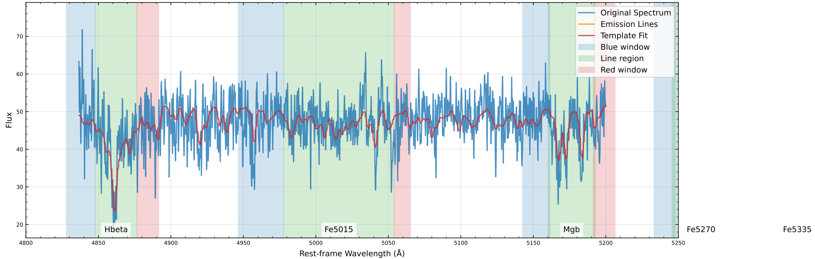
Original Data Comparison (v_star=-12.0 km/s, v_gas=28.8 km/s)
