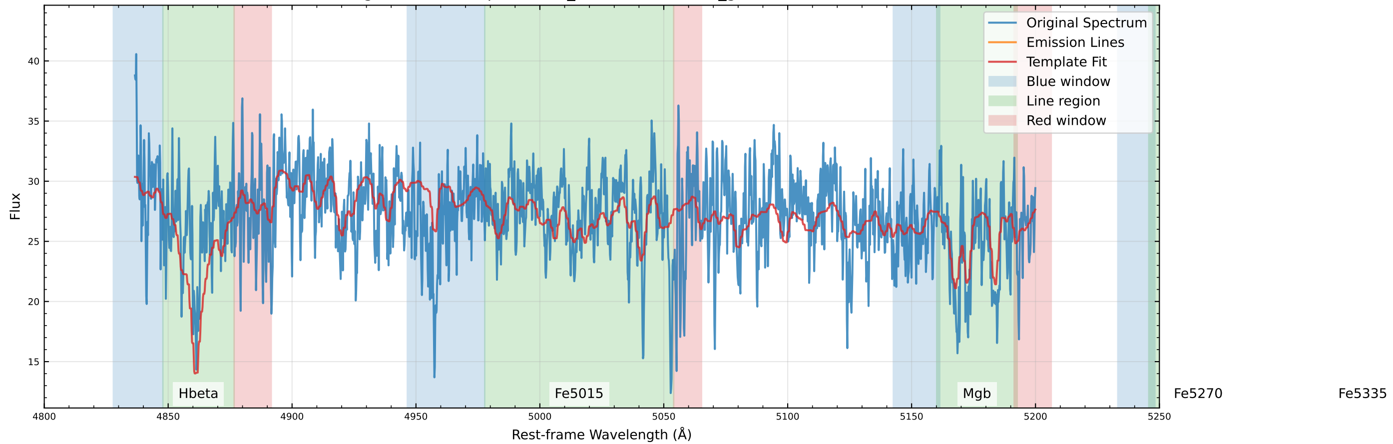
Original Data Comparison (v_star=27.6 km/s, v_gas=107.0 km/s)
