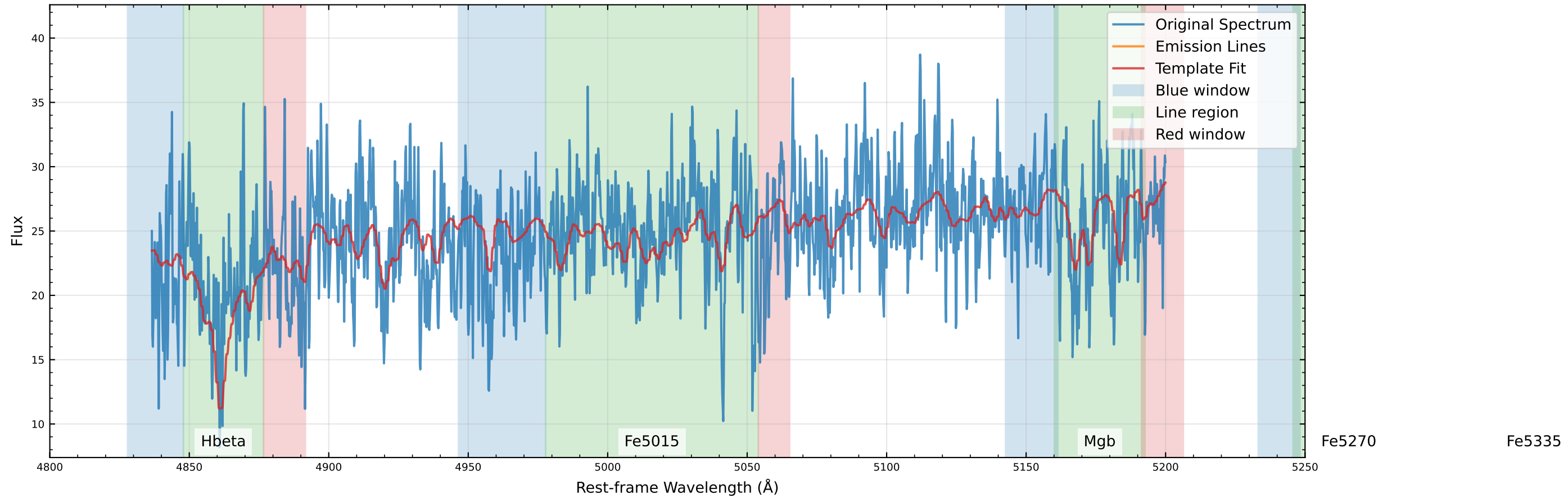
Original Data Comparison (v_star=-23.7 km/s, v_gas=29.3 km/s)
