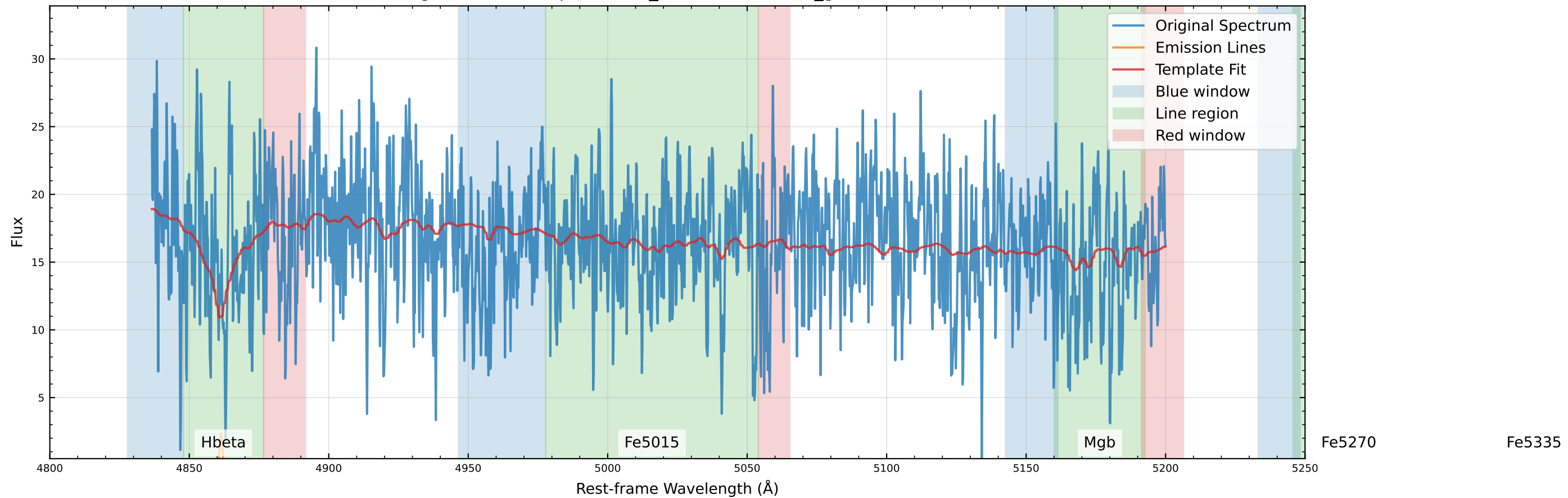
Original Data Comparison ( v_{\text{star}}=-1.7 km/s, v_{\text{gas}}=-7.5 km/s)
