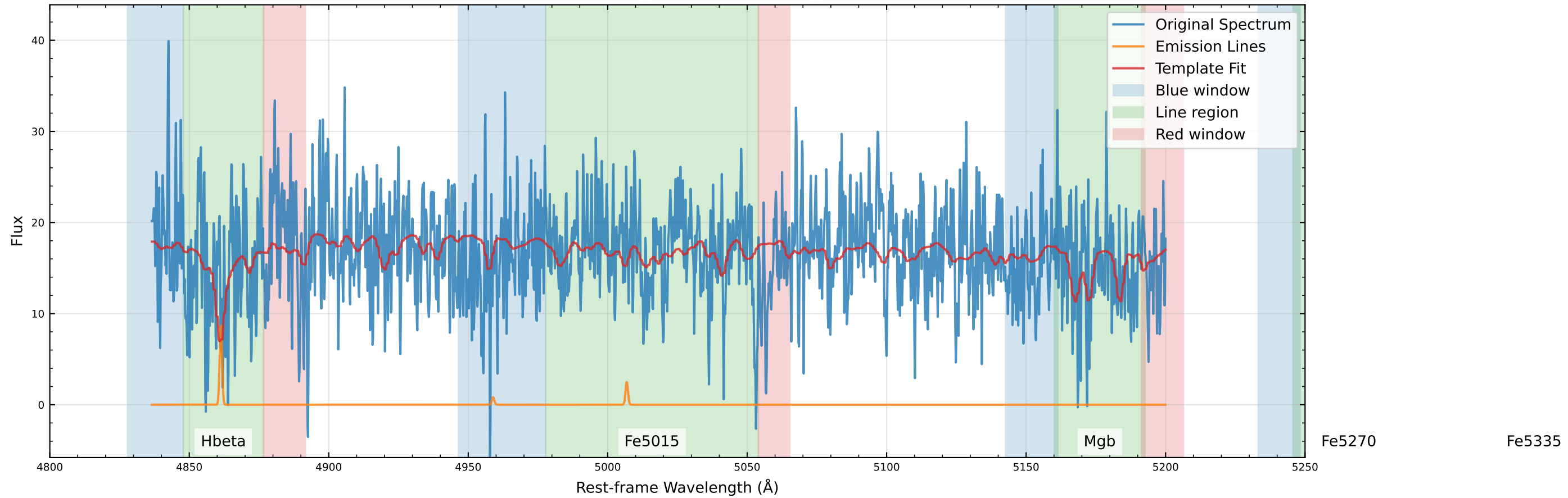
Original Data Comparison (v_star=49.0 km/s, v_gas=-35.8 km/s)
