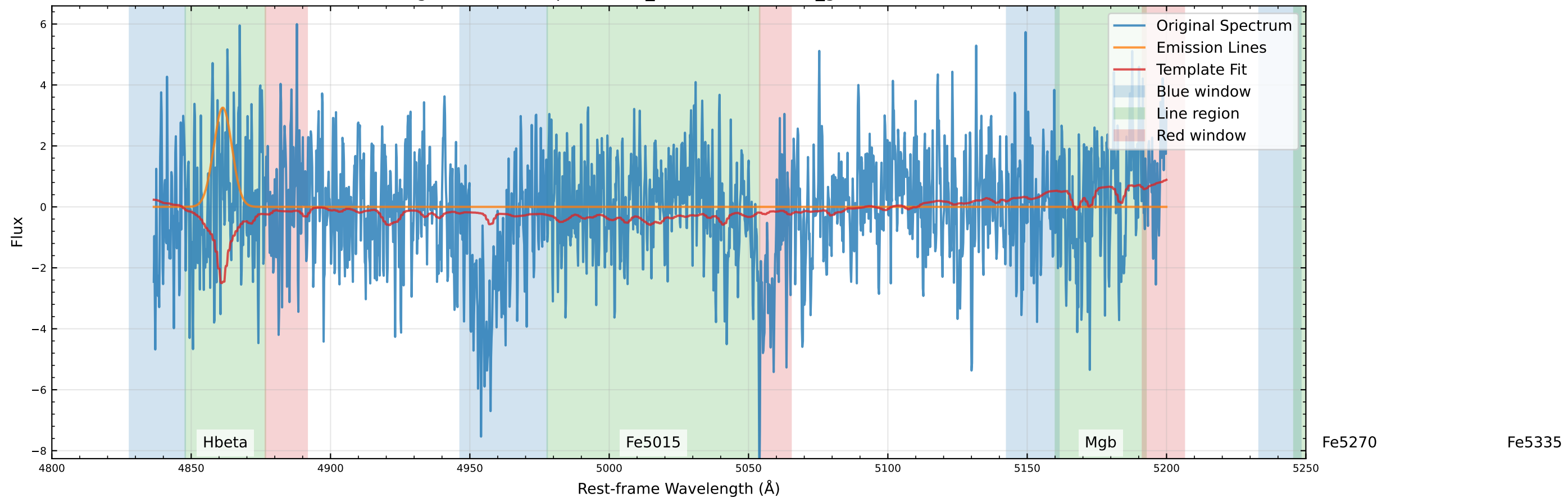
Original Data Comparison (v_star=17.1 km/s, v_gas=59.7 km/s)
