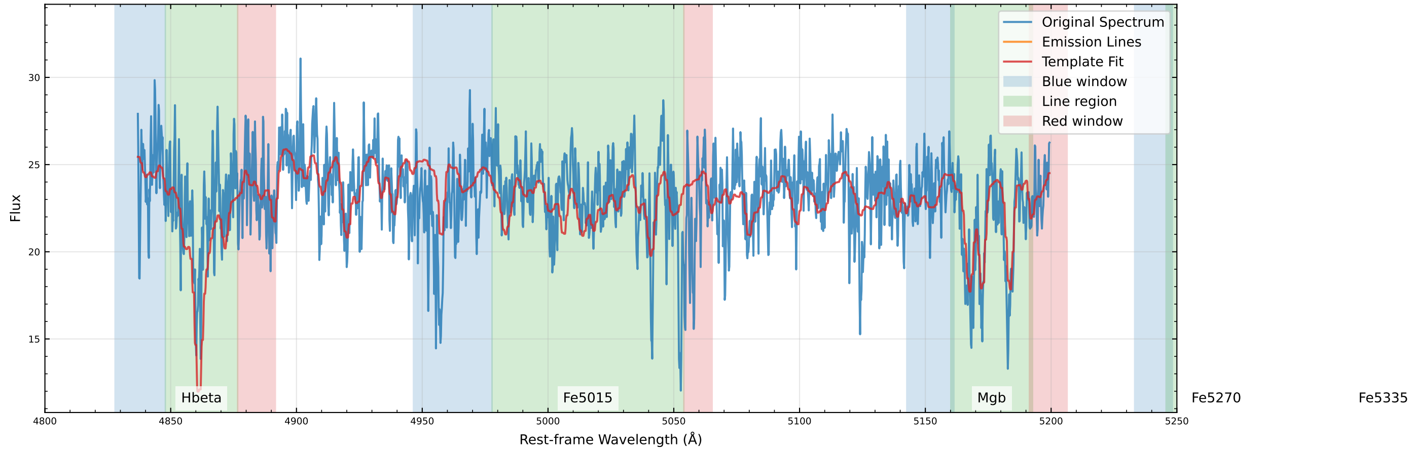
Original Data Comparison (v_star=-17.6 km/s, v_gas=32.2 km/s)
