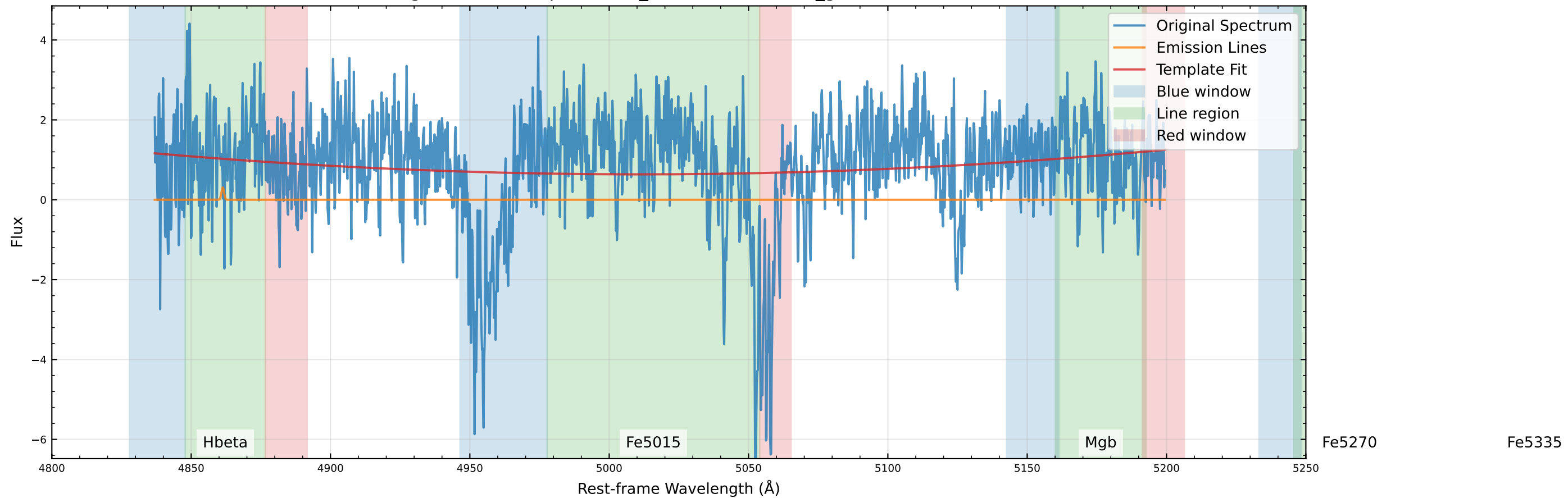
Original Data Comparison (v_star=-55.8 km/s, v_gas=-93.2 km/s)
