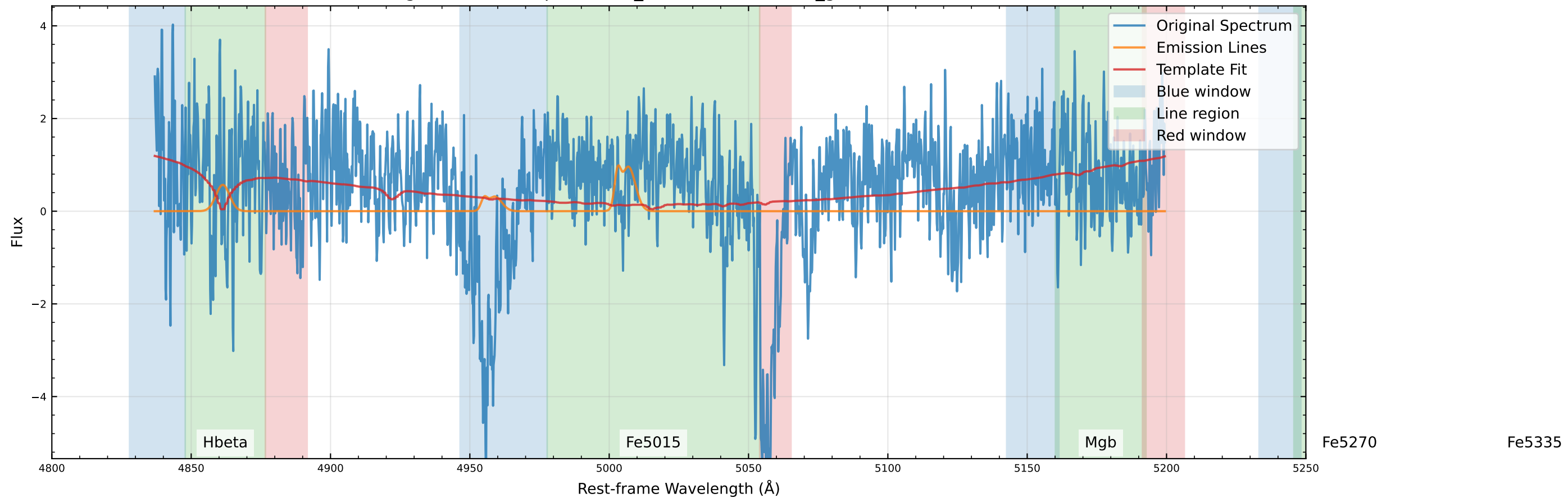
Original Data Comparison (v_star=124.8 km/s, v_gas=424.8 km/s)
