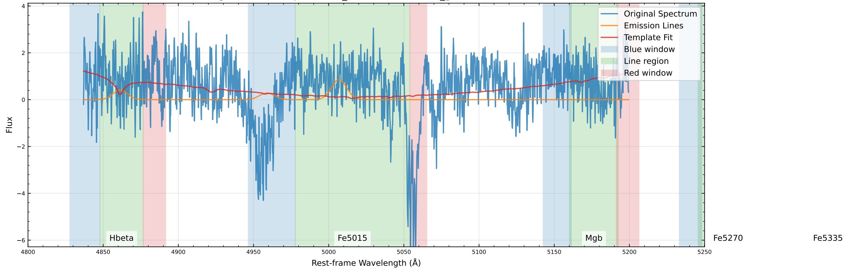
Original Data Comparison (v_star=172.6 km/s, v_gas=472.6 km/s)
