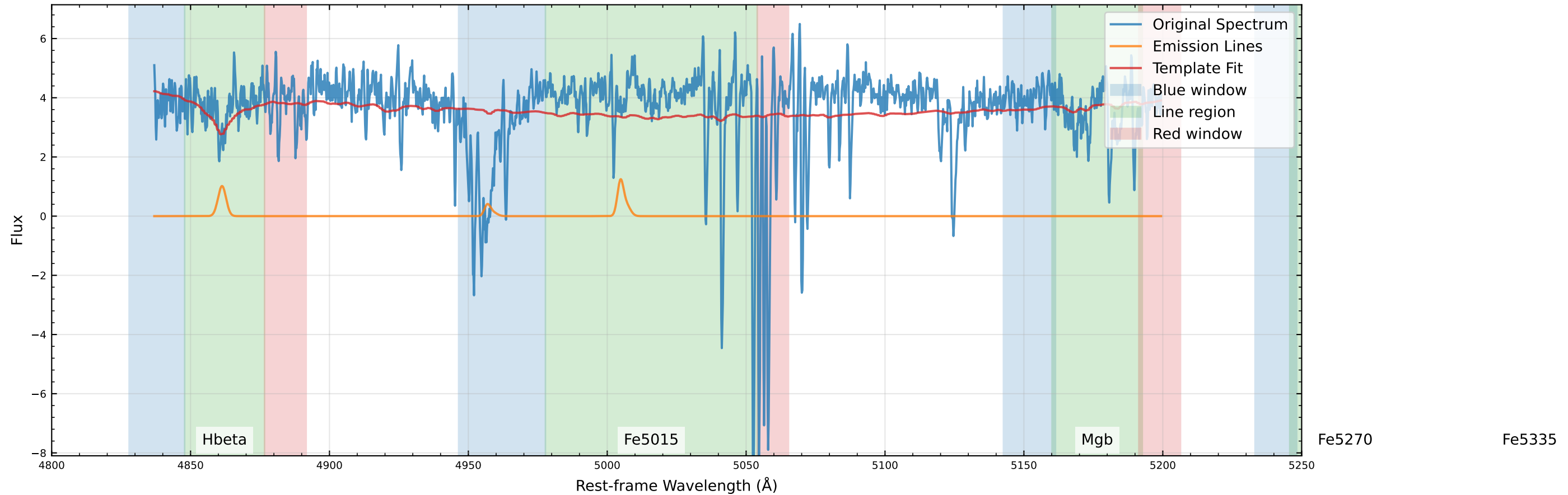
Original Data Comparison (v_star=25.8 km/s, v_gas=256.3 km/s)
