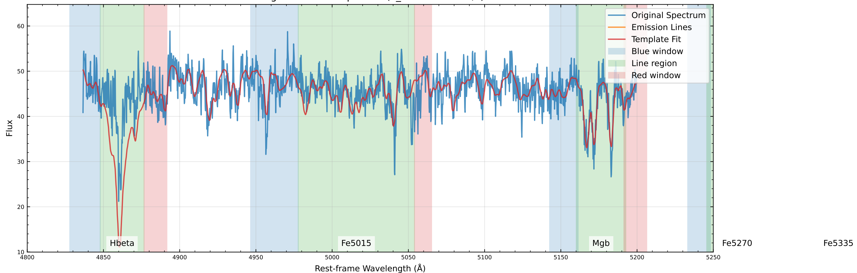
Original Data Comparison (v_star=-38.7 km/s)
