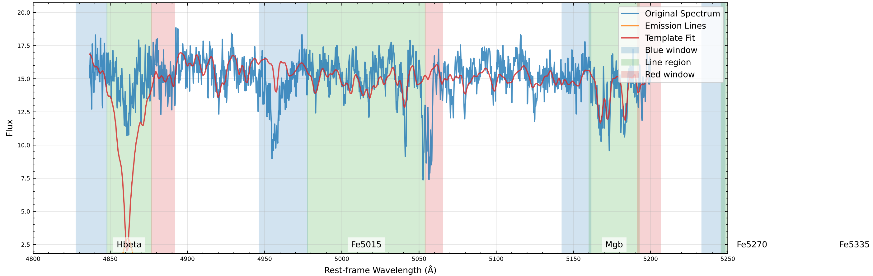
Original Data Comparison (v_star=-15.1 km/s, v_gas=-89.5 km/s)
