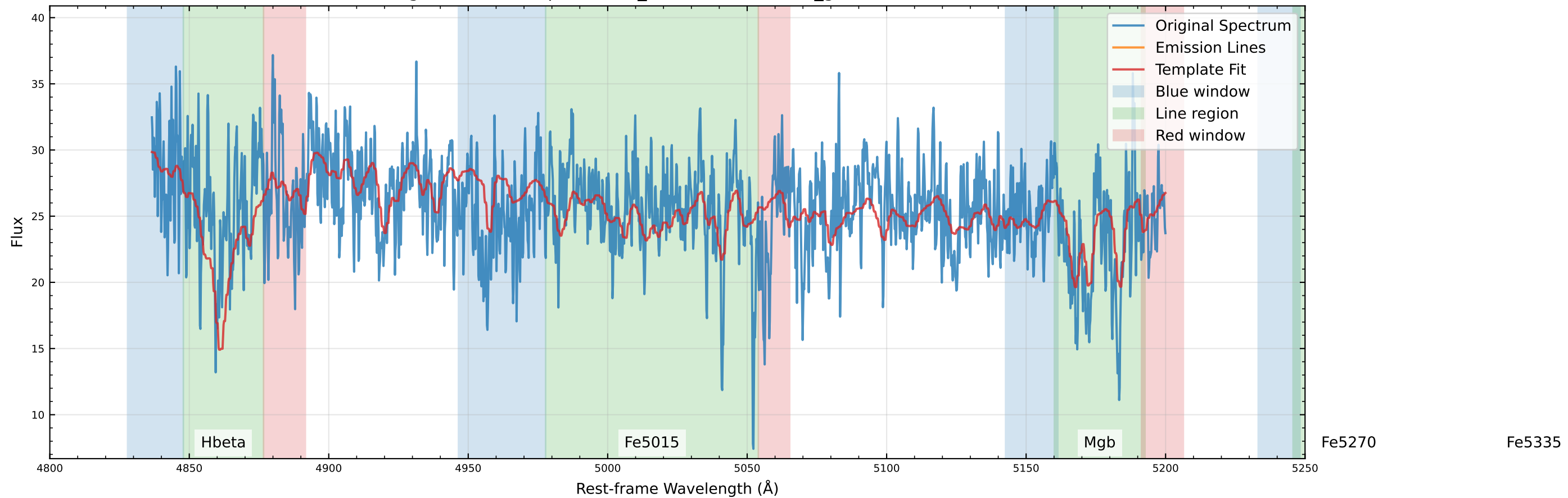
Original Data Comparison (v_star=-31.4 km/s, v_gas=-68.3 km/s)
