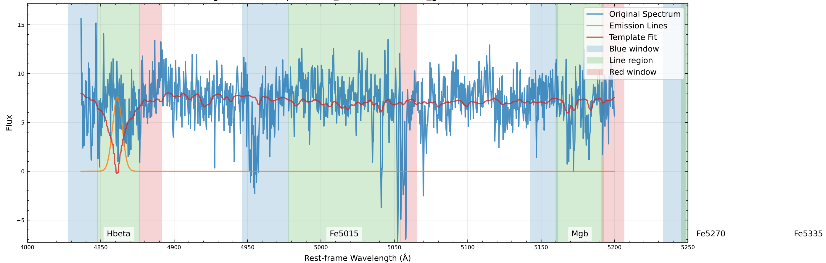
Original Data Comparison (v_star=-20.3 km/s, v_gas=-111.2 km/s)
