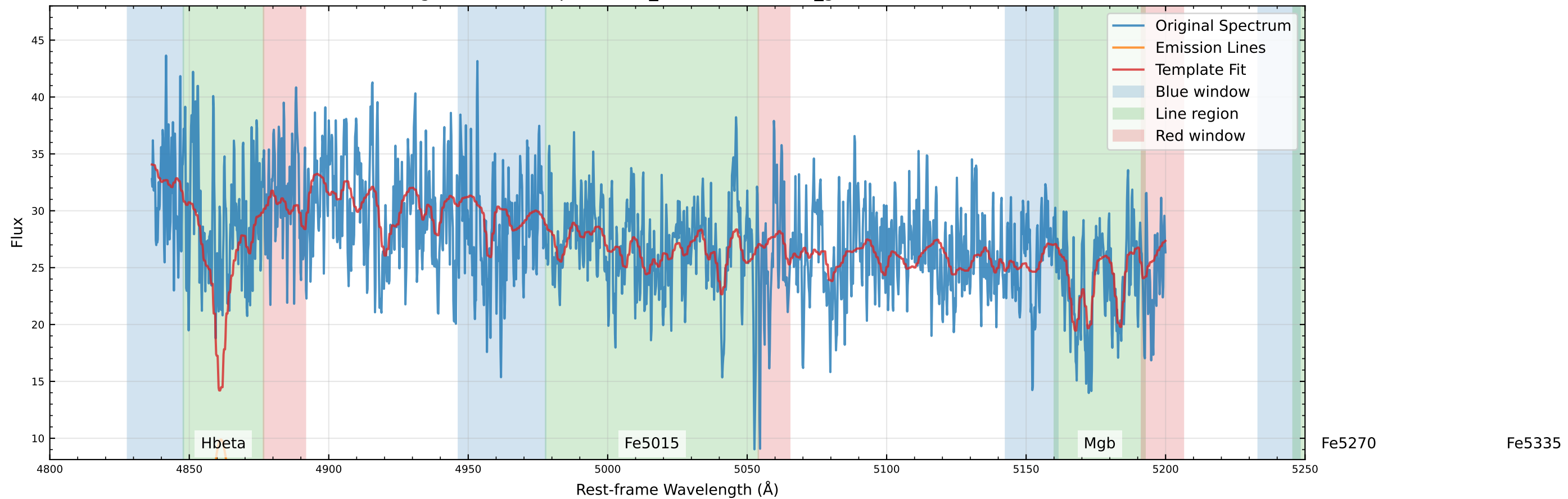
Original Data Comparison (v_star=-9.5 km/s, v_gas=-4.5 km/s)
