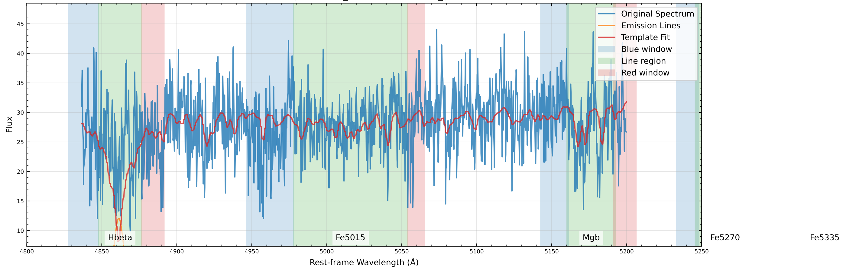
Original Data Comparison (v_star=-53.6 km/s, v_gas=-19.7 km/s)
