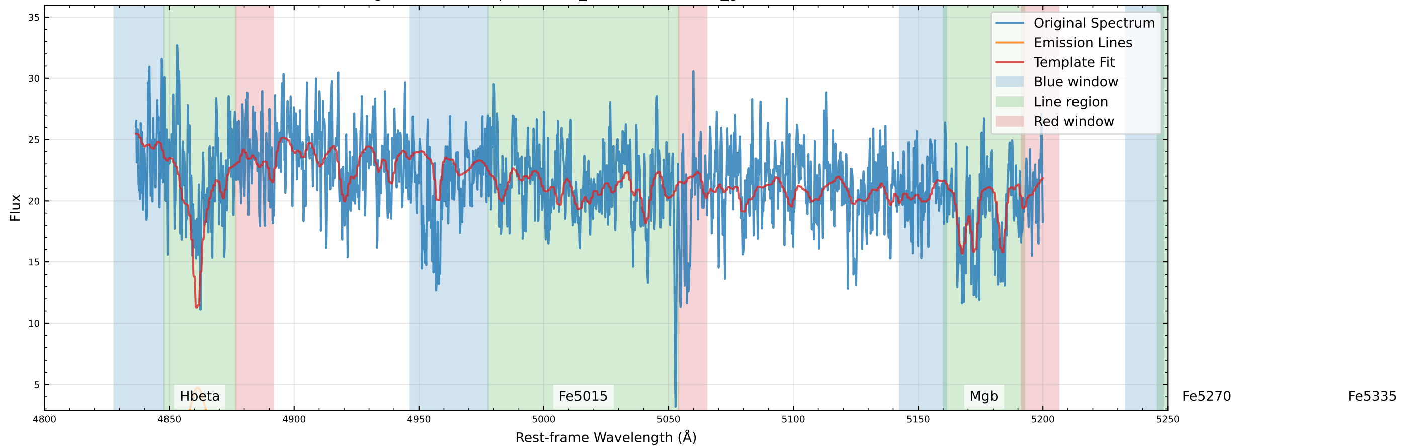
Original Data Comparison (v_star=7.8 km/s, v_gas=-45.6 km/s)
