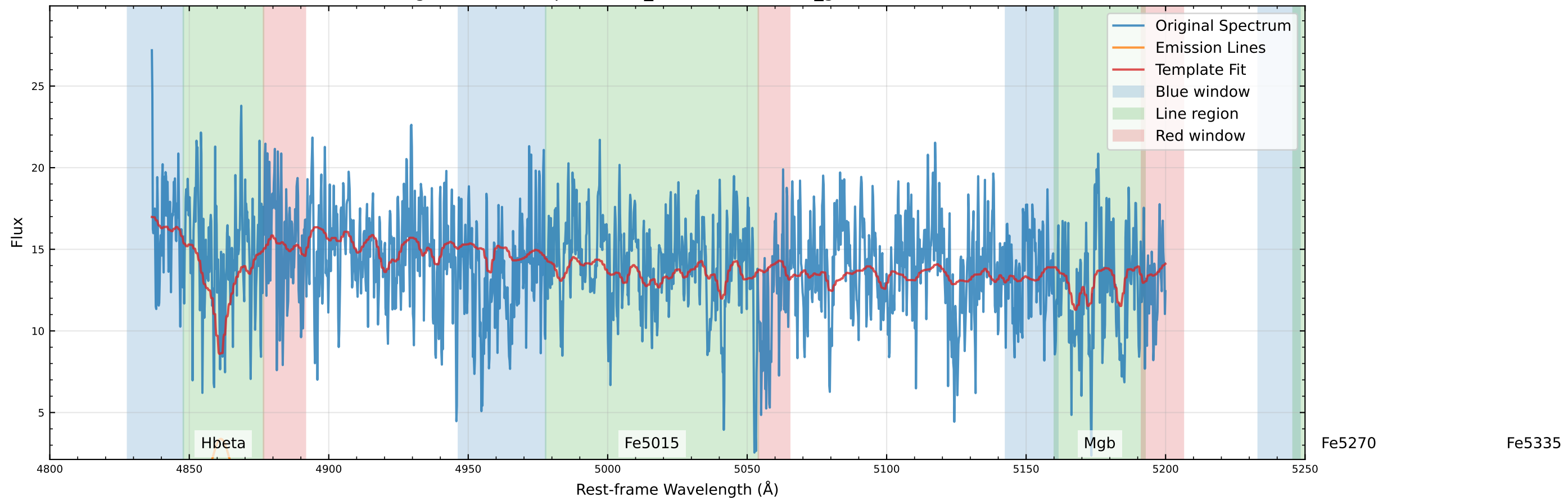
Original Data Comparison ( v_{\text{star}}=10.3 km/s, v_{\text{gas}}=50.7 km/s)
