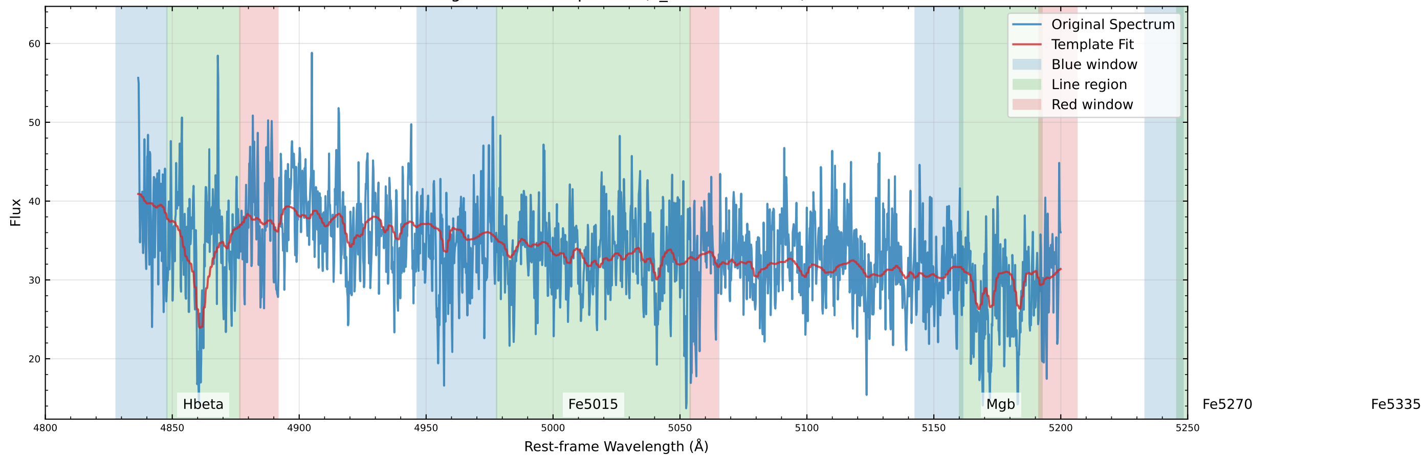
Original Data Comparison (v_star=-26.3 km/s)
