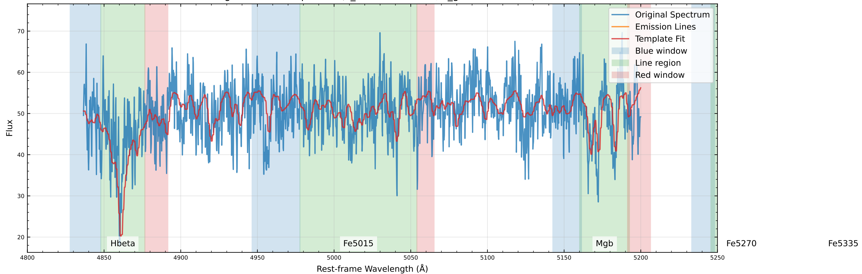
Original Data Comparison (v_star=-58.4 km/s, v_gas=-74.9 km/s)
