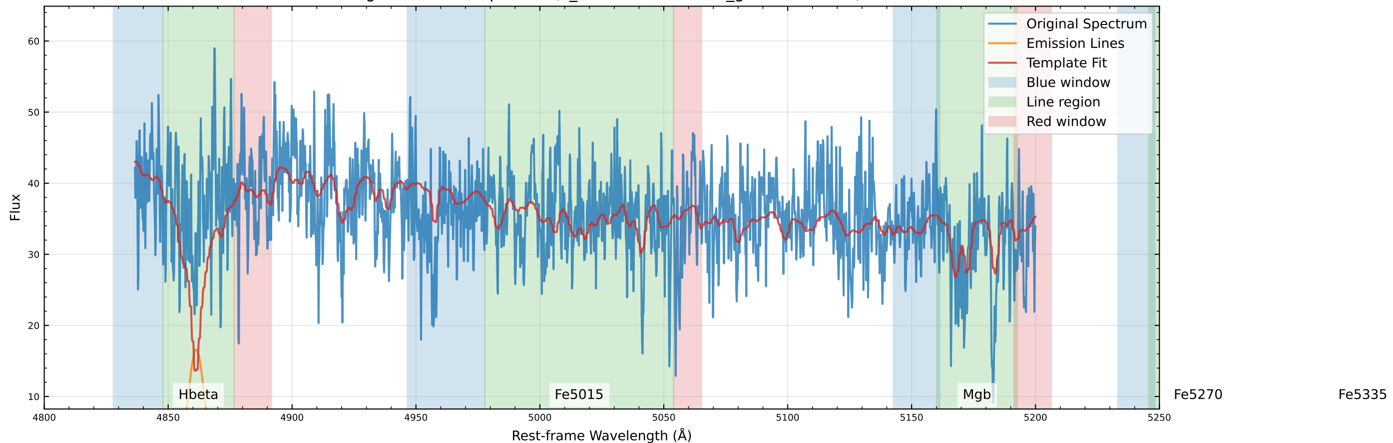
Original Data Comparison (v_star=-19.7 km/s, v_gas=53.3 km/s)
