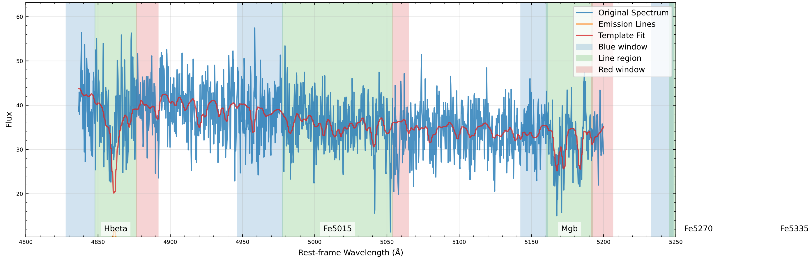
Original Data Comparison (v_star=-17.1 km/s, v_gas=56.1 km/s)
