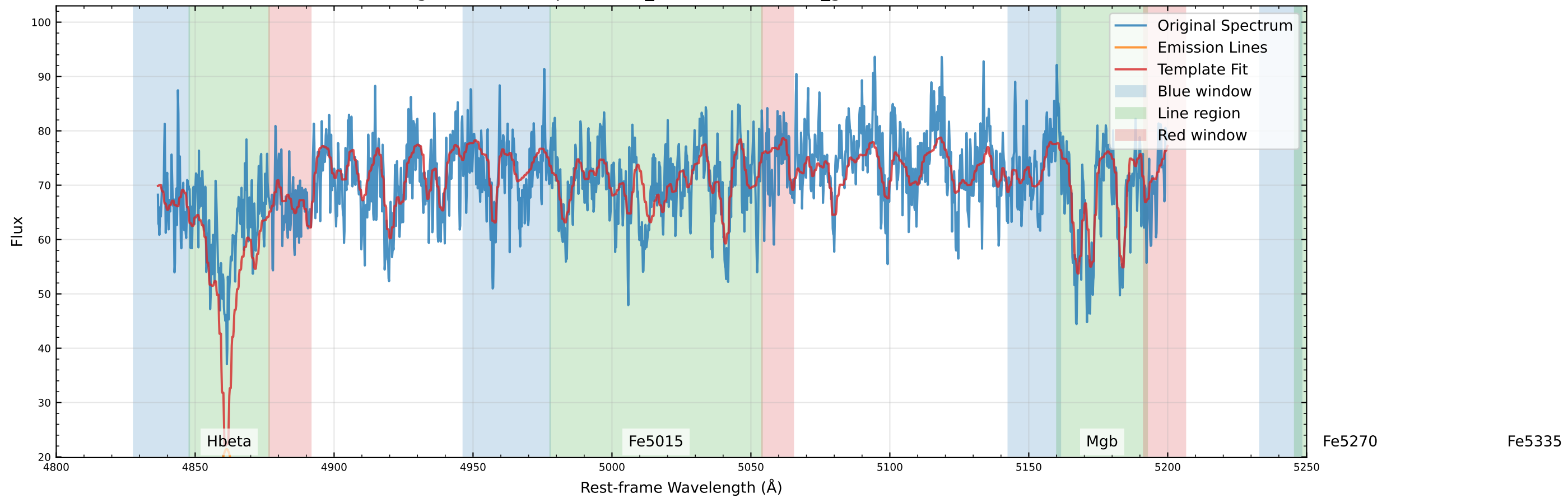
Original Data Comparison (v_star=-16.3 km/s, v_gas=13.6 km/s)
