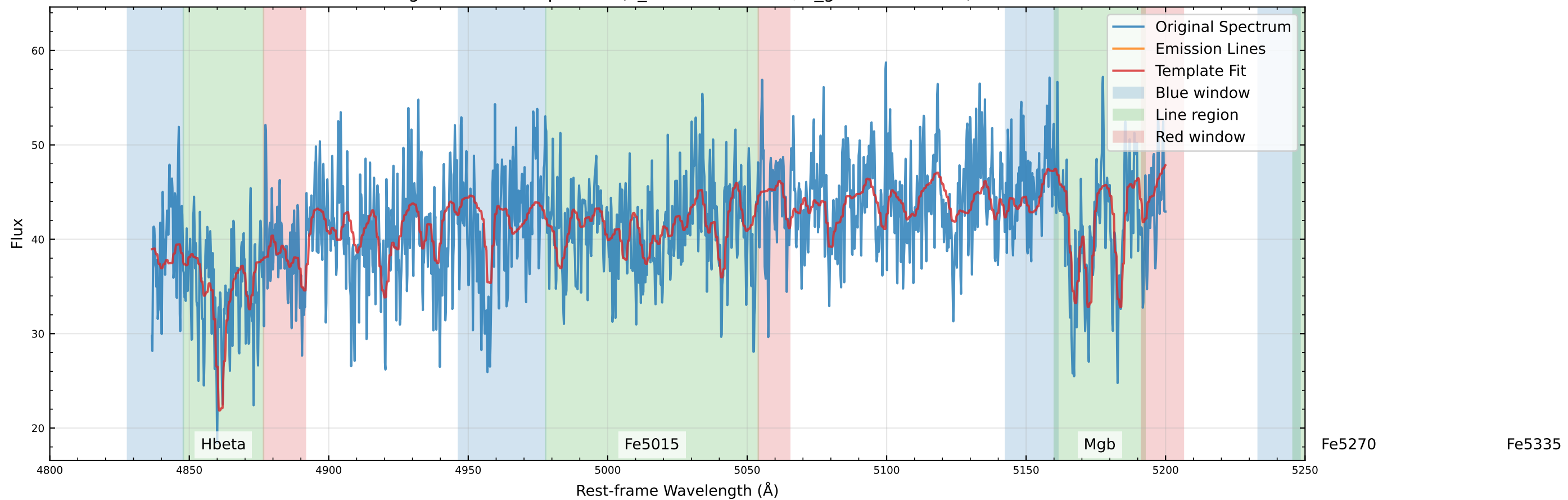
Original Data Comparison (v_star=-28.7 km/s, v_gas=-26.3 km/s)
