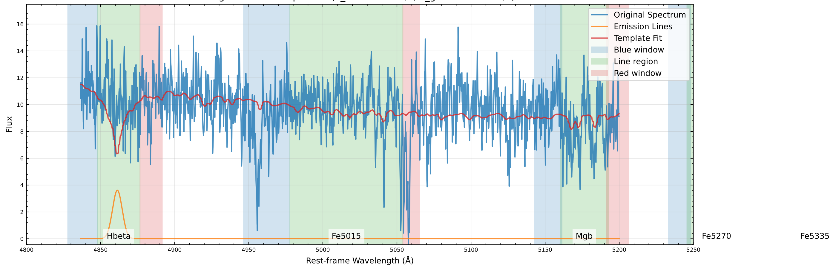
Original Data Comparison (v_star=9.6 km/s, v_gas=-120.4 km/s)
