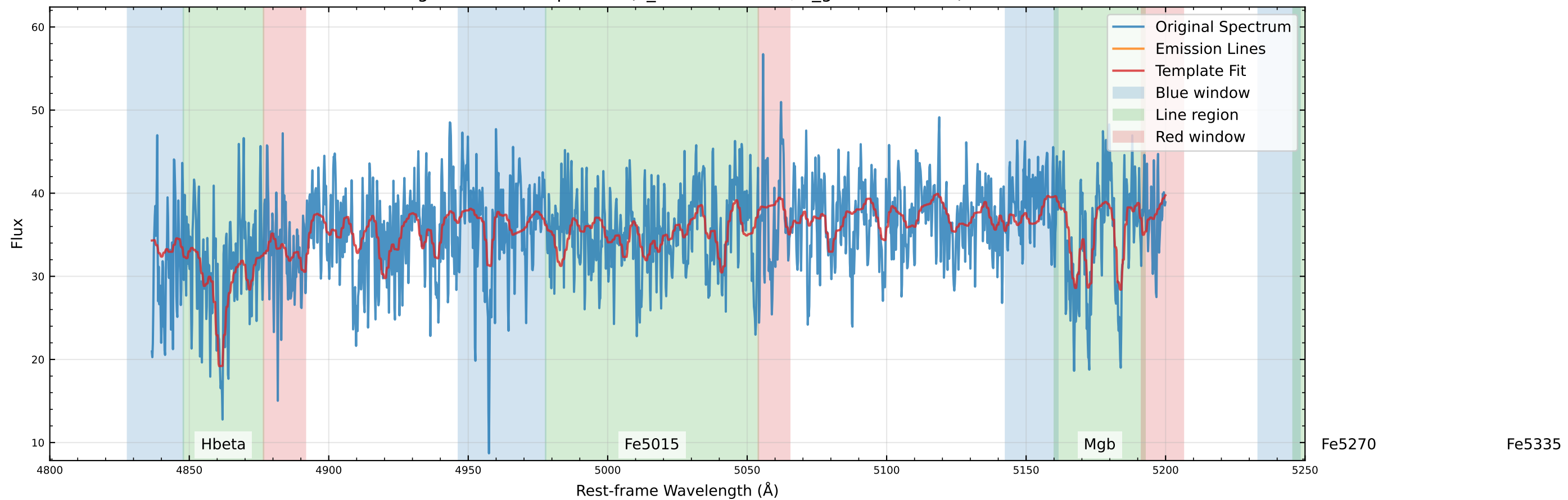
Original Data Comparison (v_star=-9.8 km/s, v_gas=28.3 km/s)
