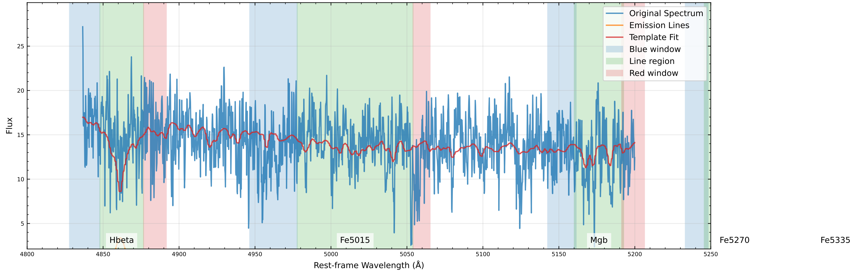
Original Data Comparison (v_star=10.3 km/s, v_gas=50.7 km/s)
