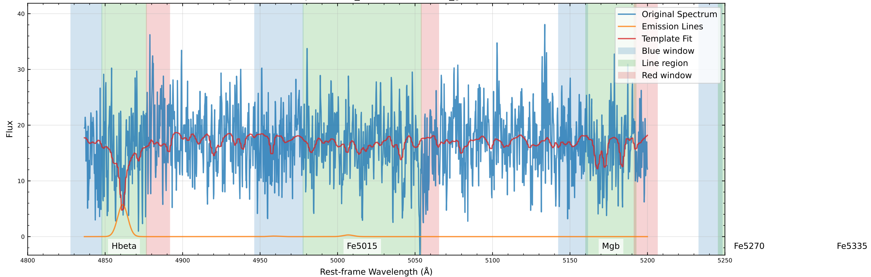
Original Data Comparison (v_star=51.7 km/s, v_gas=171.5 km/s)
