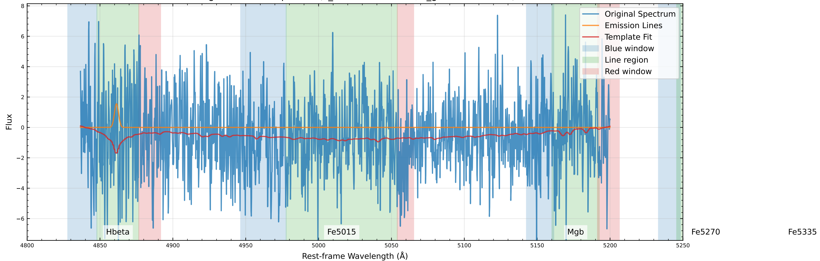
Original Data Comparison (v_star=-257.9 km/s, v_gas=-130.4 km/s)
