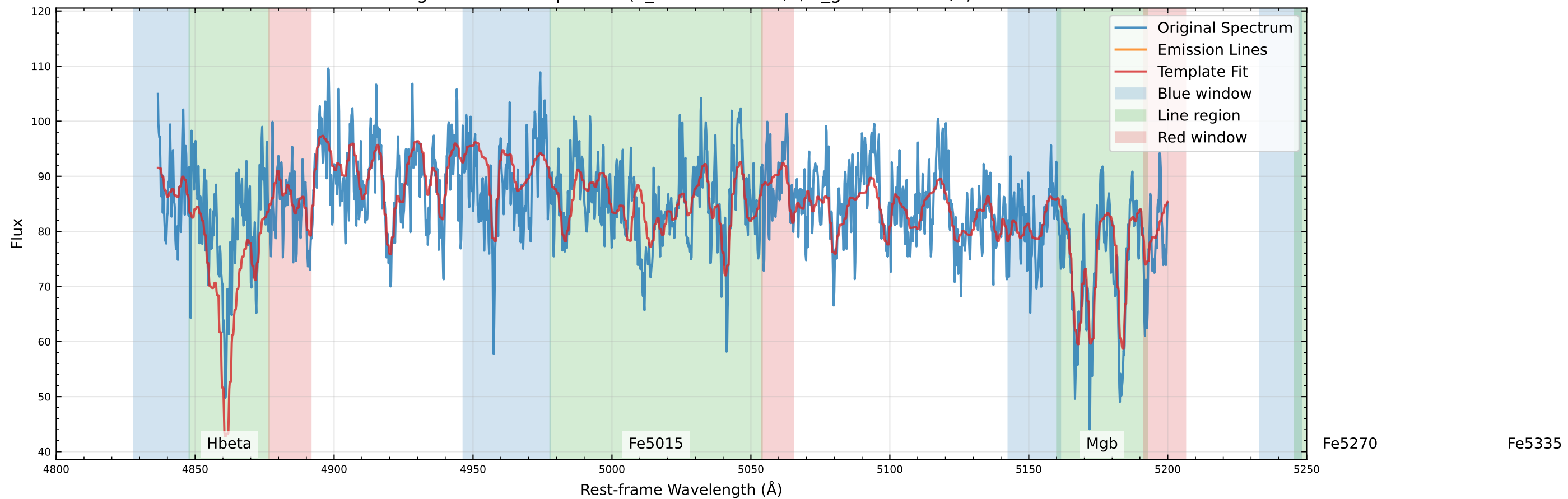
Original Data Comparison (v_star=-11.0 km/s, v_gas=17.0 km/s)
