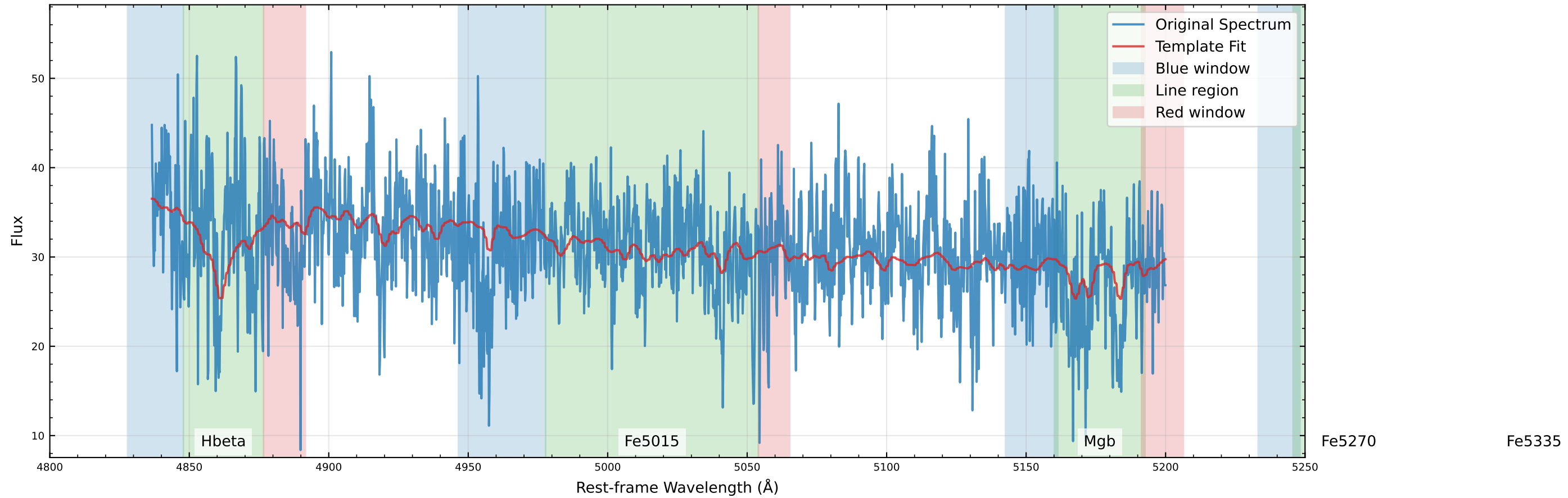
Original Data Comparison (v_star=-41.2 km/s)
