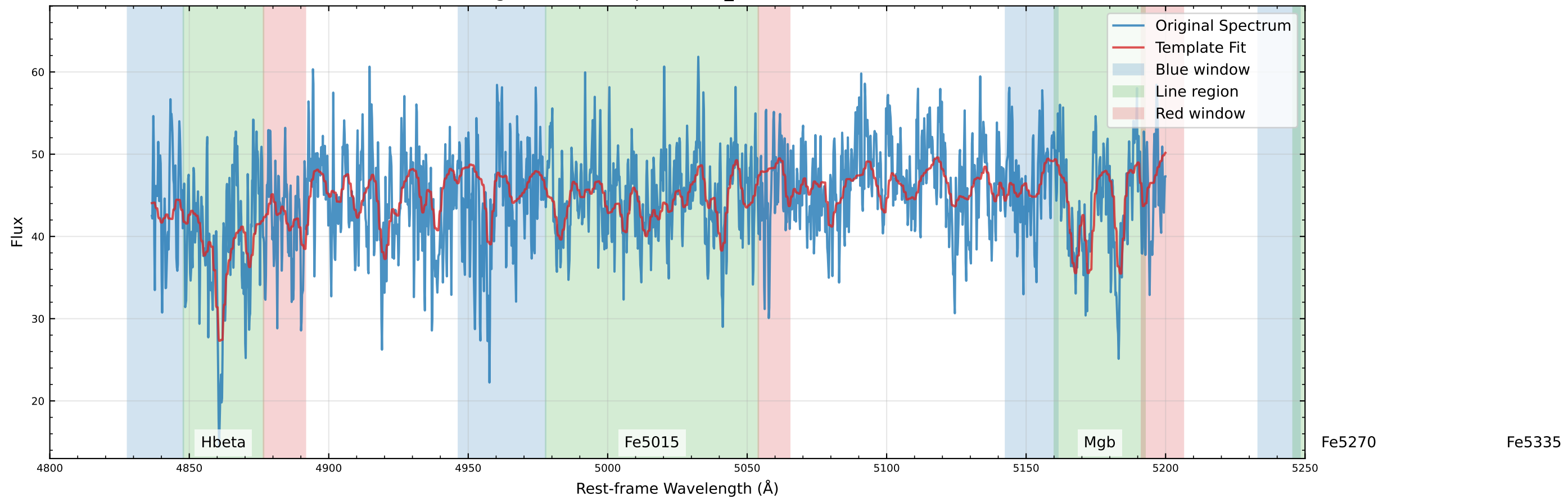
Original Data Comparison (v_star=-34.6 km/s)
