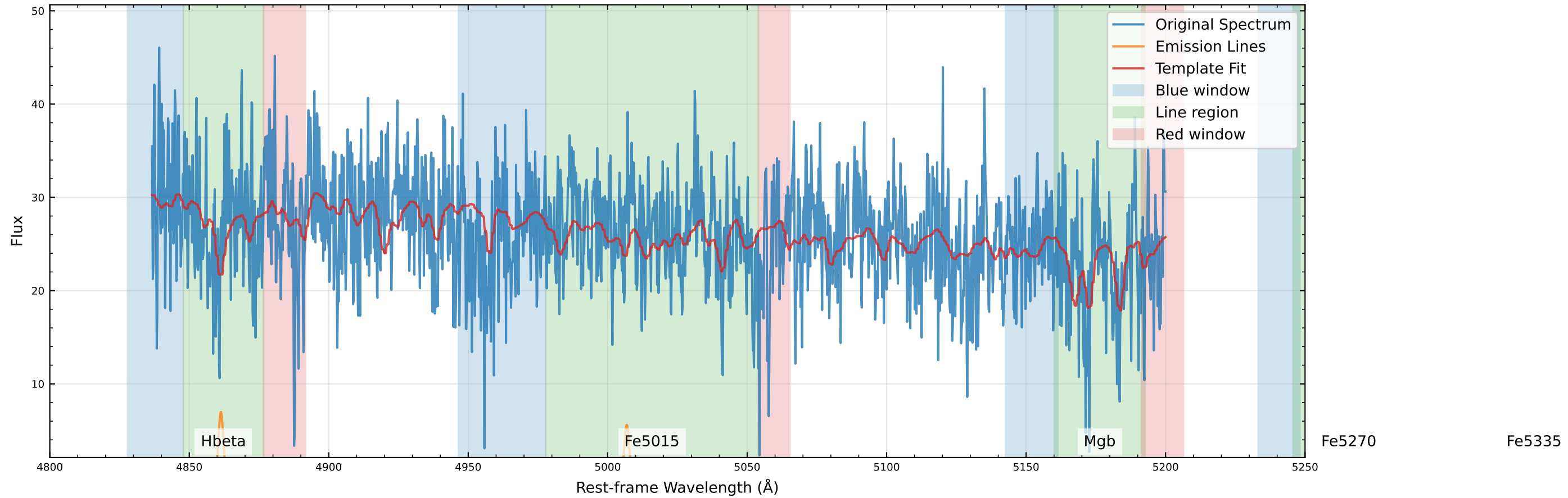
Original Data Comparison (v_star=-43.9 km/s, v_gas=113.3 km/s)
