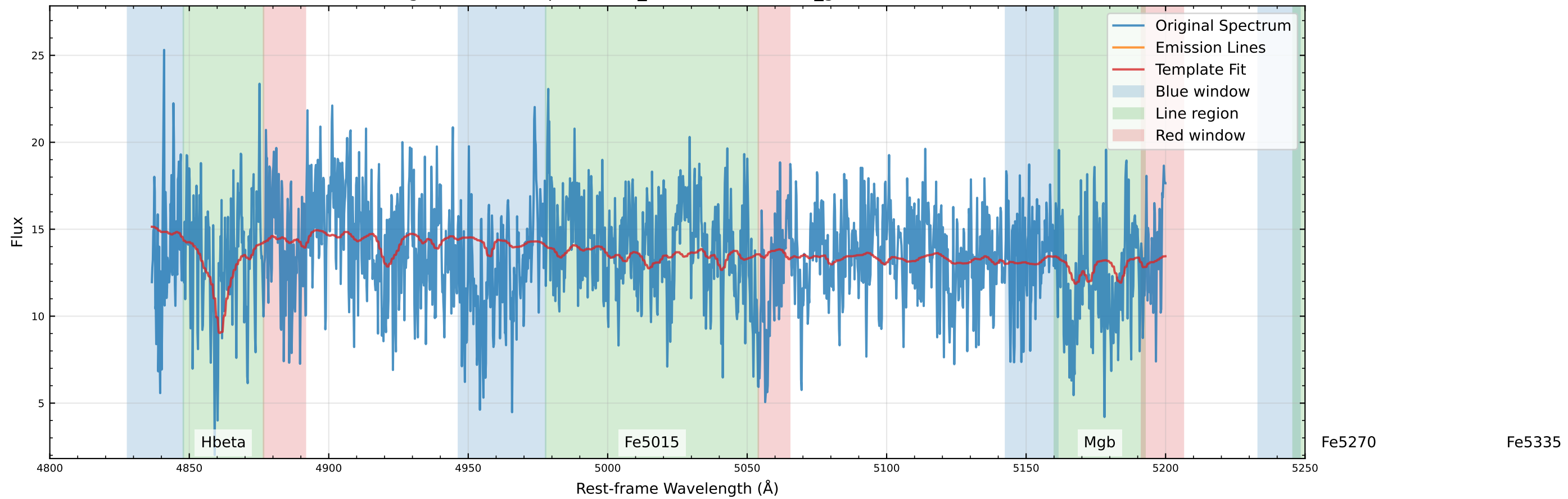
Original Data Comparison (v_star=-72.7 km/s, v_gas=-57.1 km/s)
