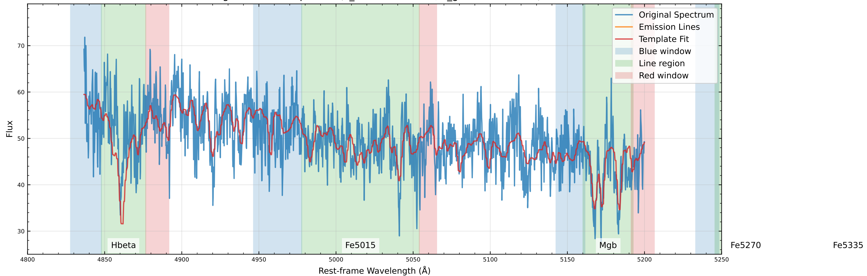
Original Data Comparison ( v_{\text{star}}=-28.5 km/s, v_{\text{gas}}=-147.7 km/s)
