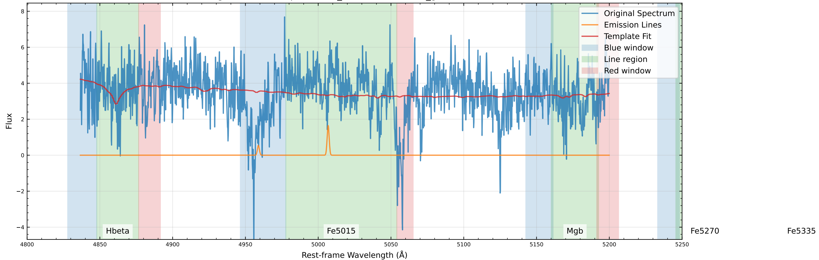
Original Data Comparison (v_star=62.5 km/s, v_gas=95.9 km/s)
