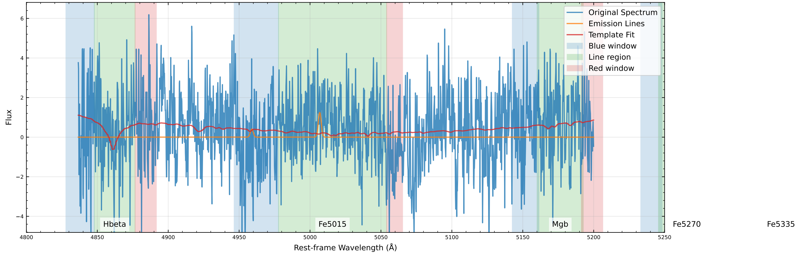
Original Data Comparison (v_star=-10.4 km/s, v_gas=-27.2 km/s)
